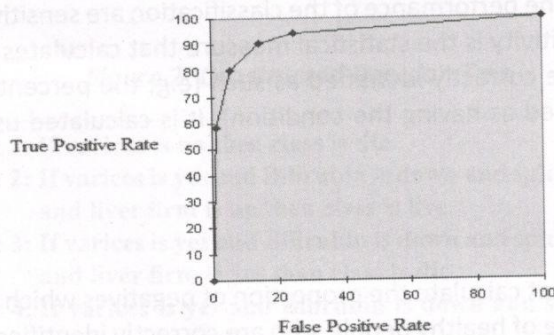
Figure 4. ROC Curve
