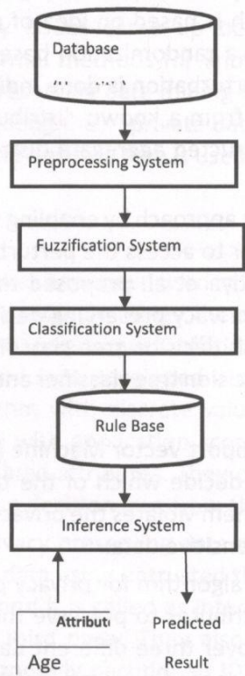
Figure 1. Proposed System Architecture Hepatitis Database
